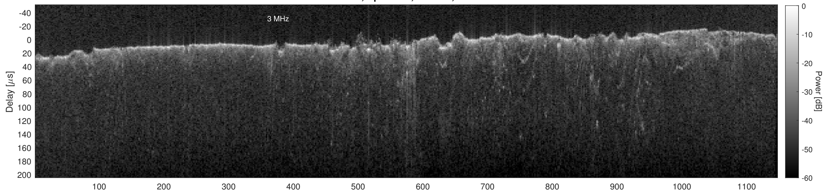
Orbit 13174, Cluttergram
