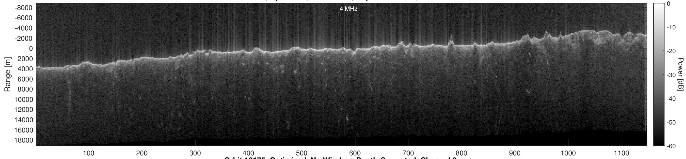
Orbit 13175, Optimized, No Window, Depth-Corrected, Channel 2
