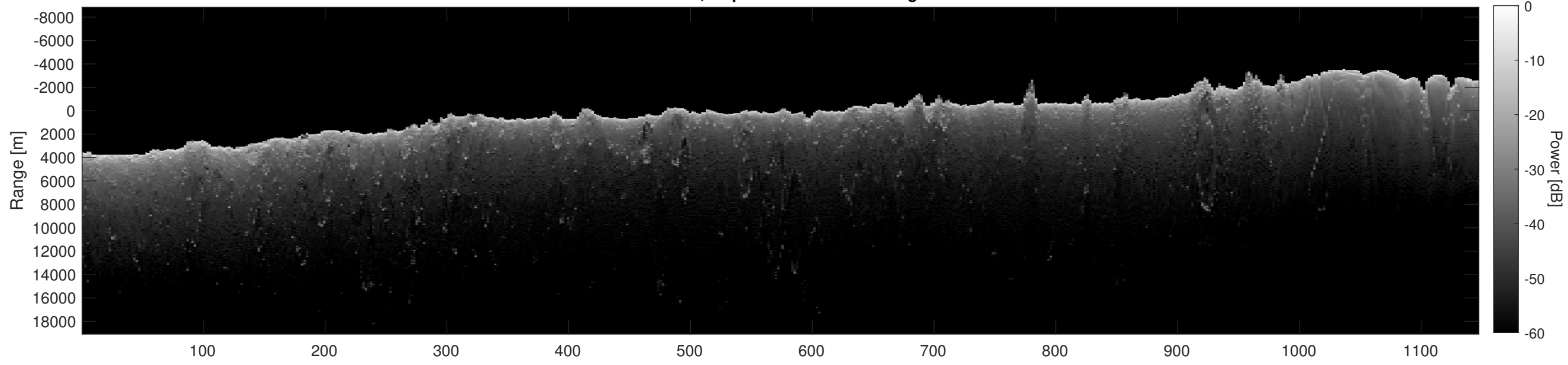
Orbit 13175, Depth-Corrected Cluttergram
