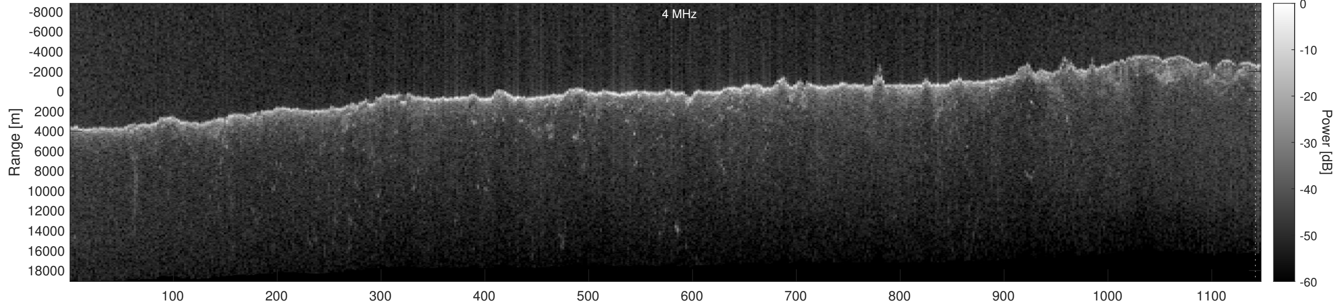
Orbit 13175, Optimized, Window, Depth-Corrected, Channel 2
