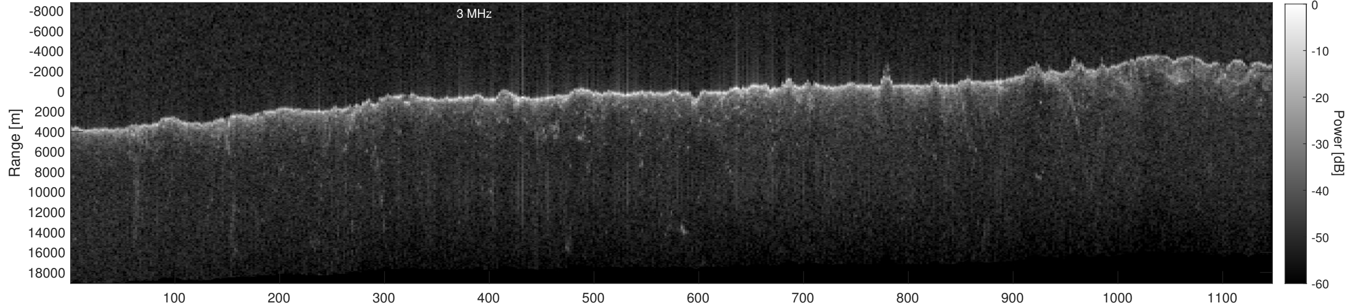
Orbit 13175, Depth-Corrected Cluttergram
