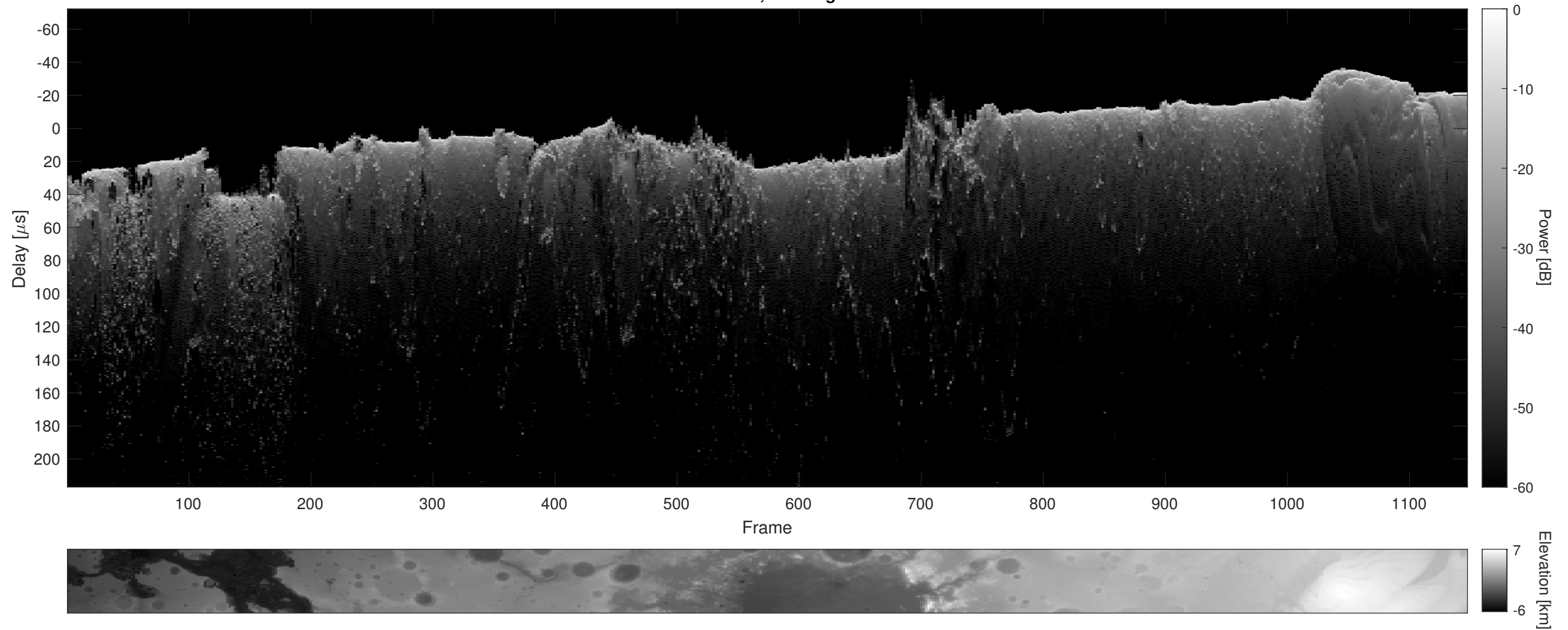
Orbit 13186, Cluttergram
