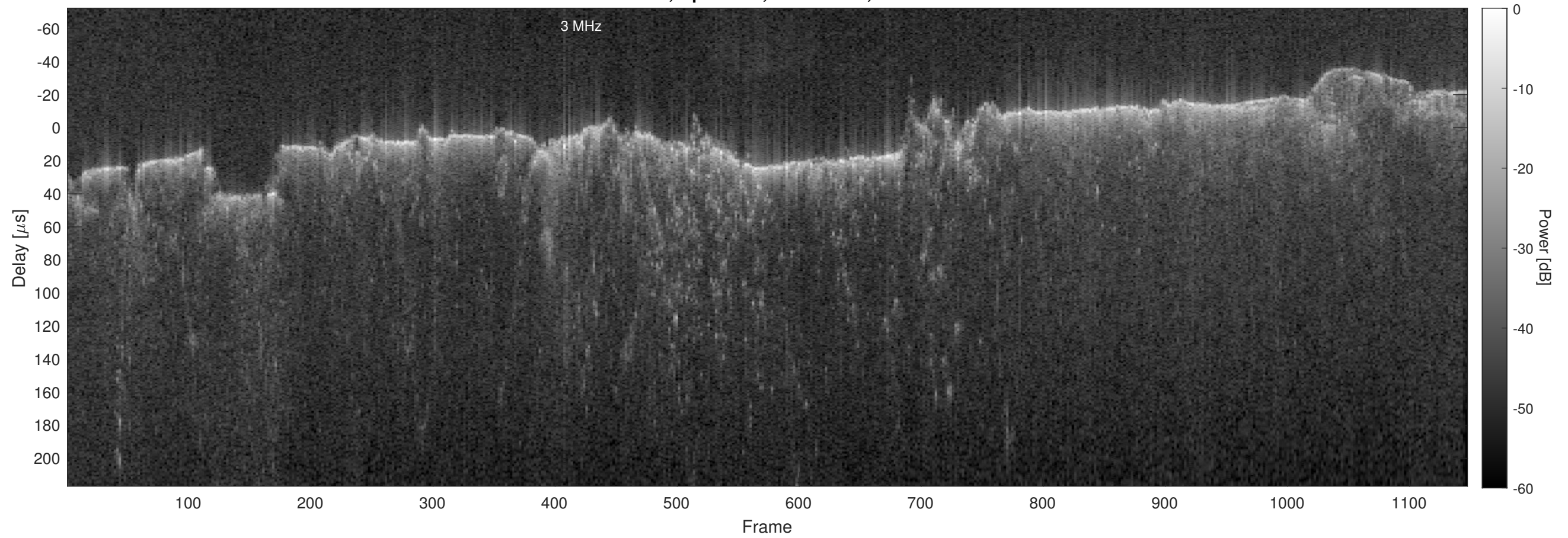
Orbit 13186, Optimized, No Window, Channel 2
