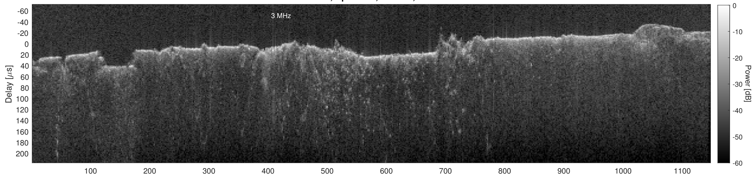
Orbit 13186, Cluttergram
