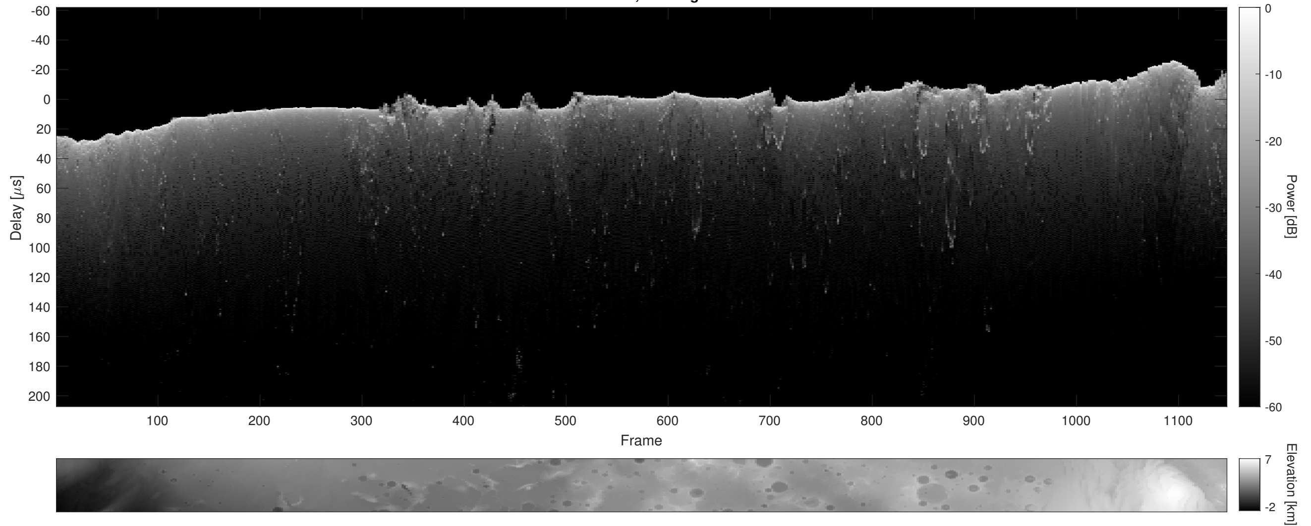
Orbit 13187, Cluttergram
