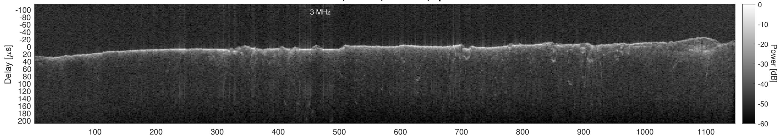
Orbit 13187, Cluttergram
