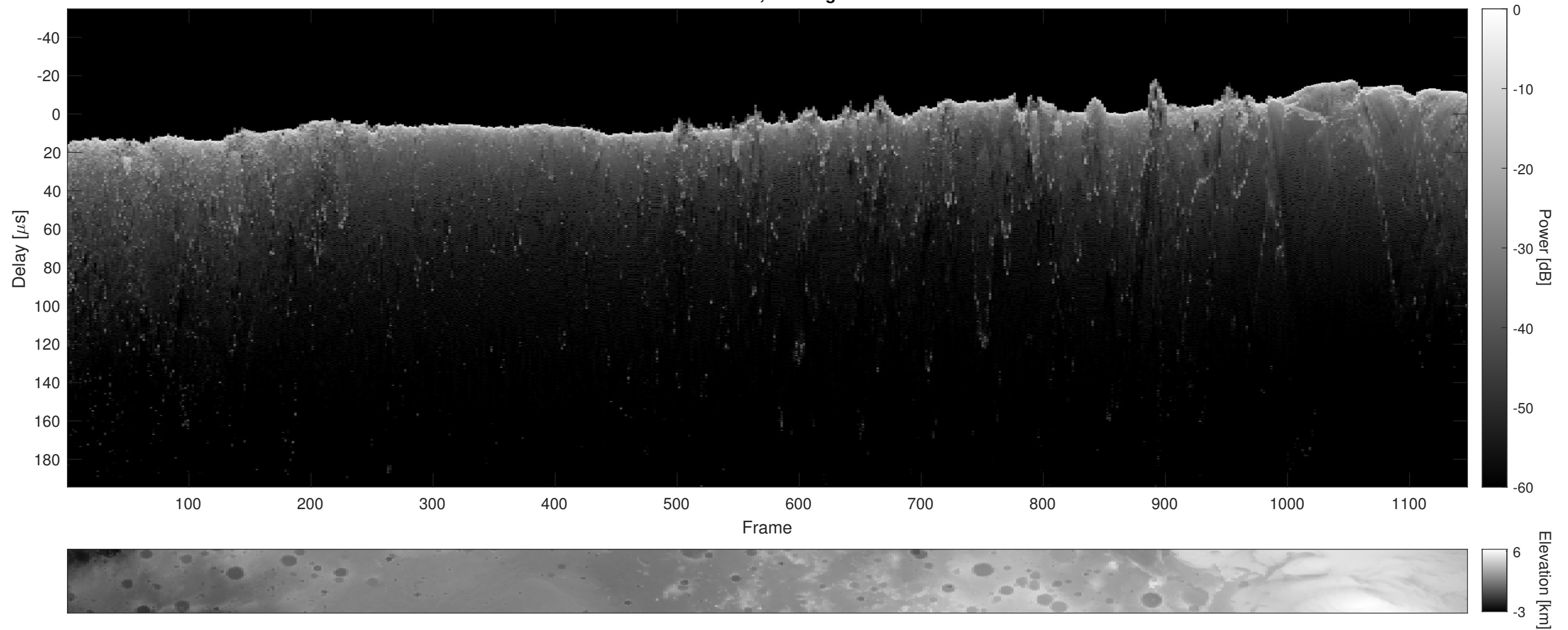
Orbit 13188, Cluttergram
