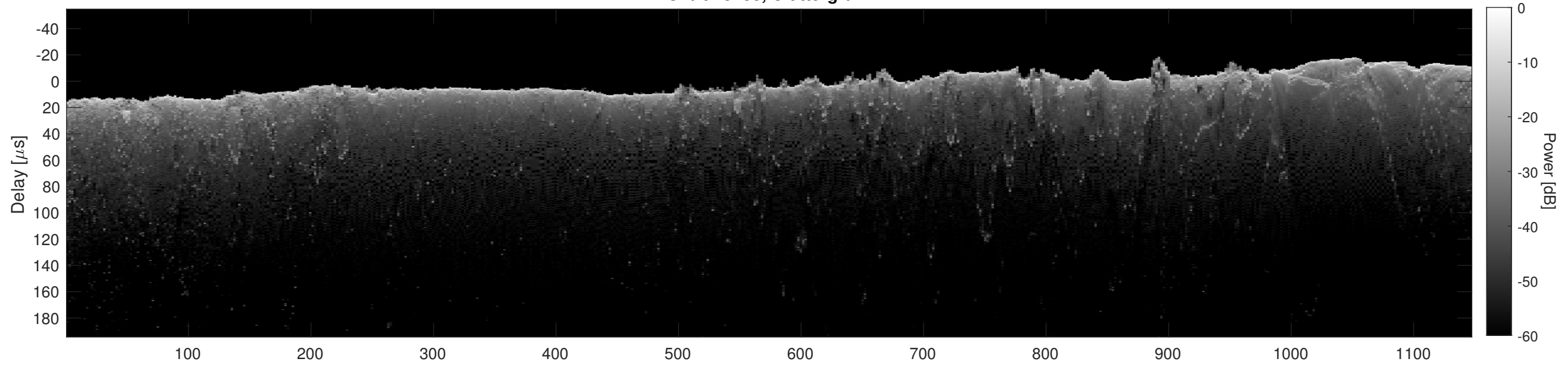
Orbit 13188, Cluttergram
