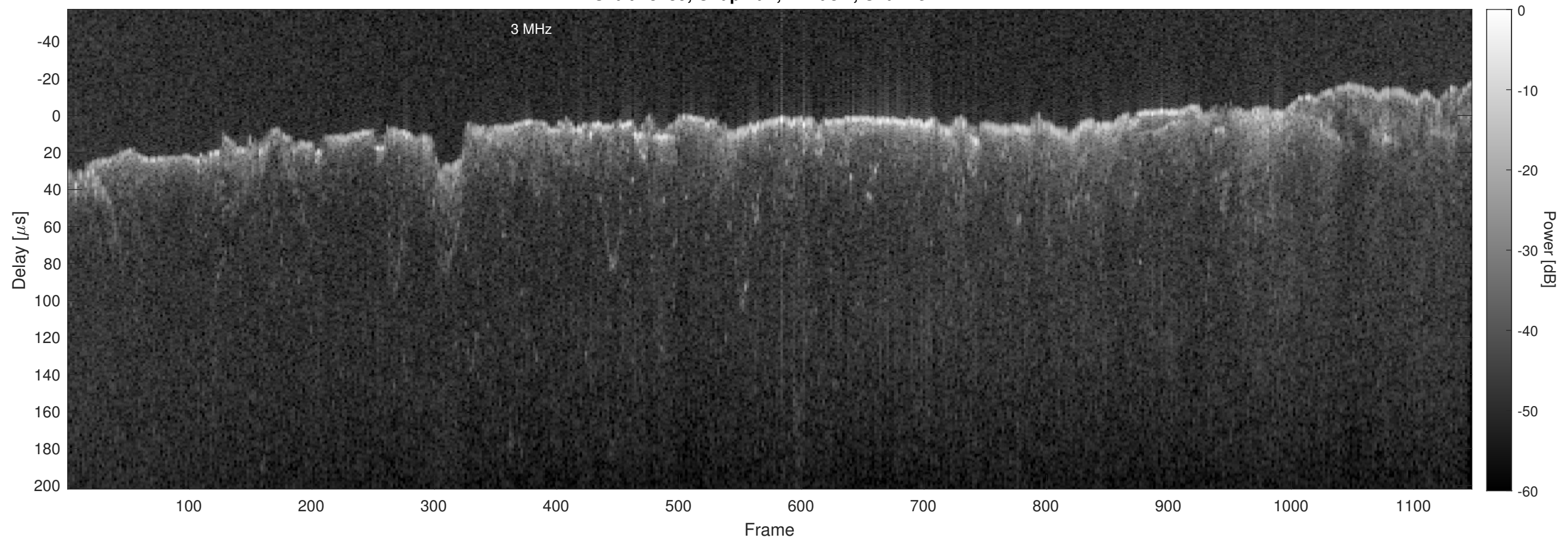
Orbit 13189, Chapman, Window, Channel 2
