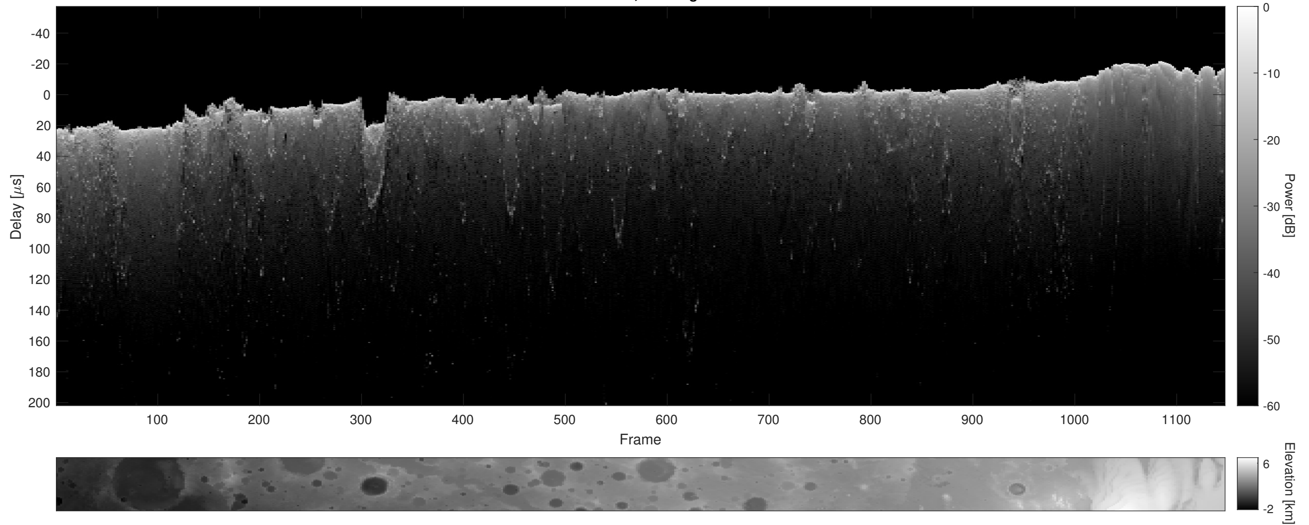
Orbit 13189, Cluttergram
