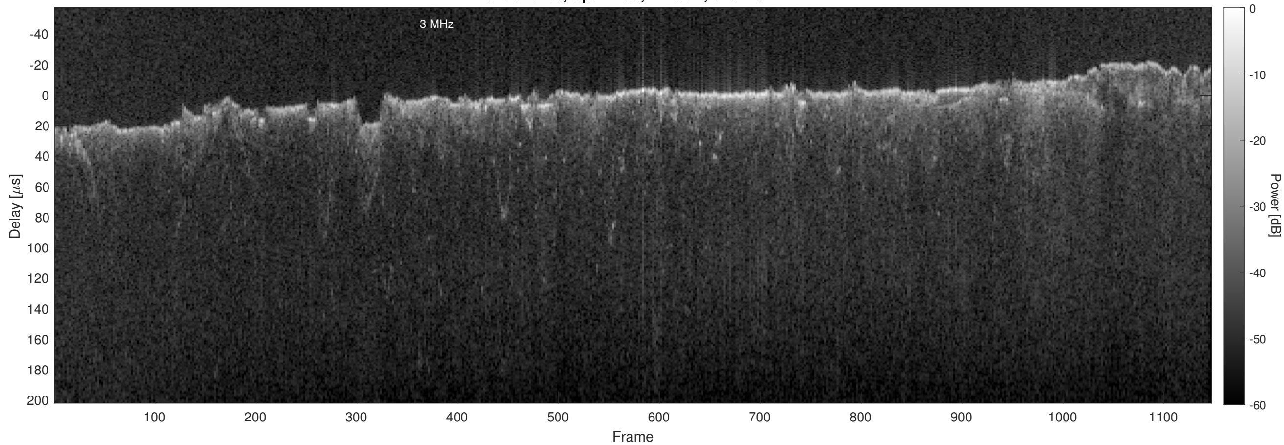
Orbit 13189, Optimized, Window, Channel 2
