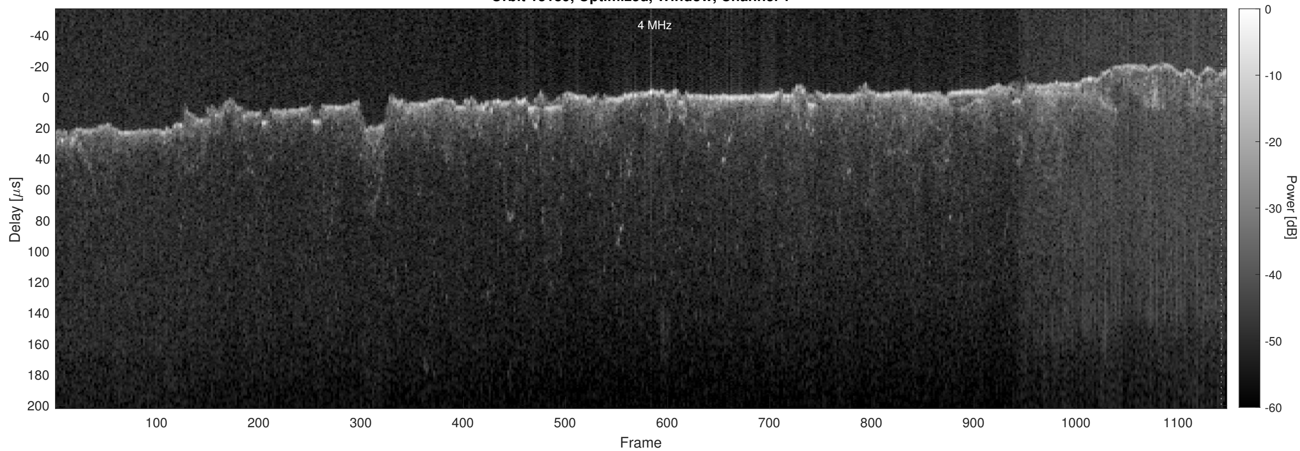
Orbit 13189, Optimized, Window, Channel 2
