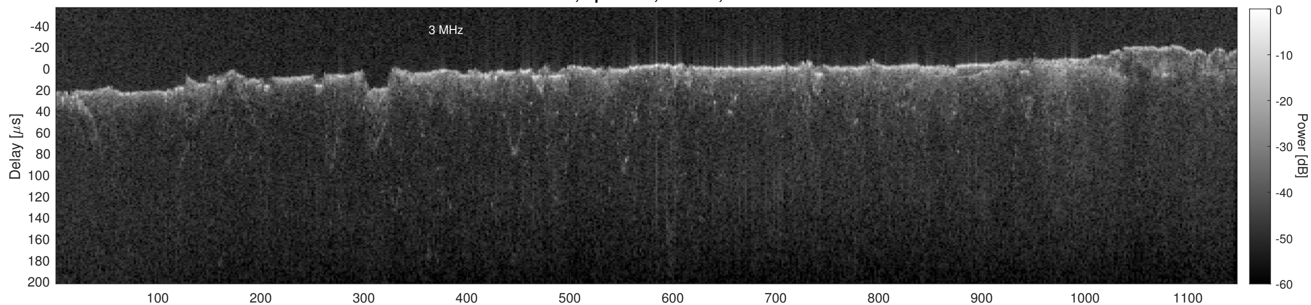
Orbit 13189, Cluttergram
