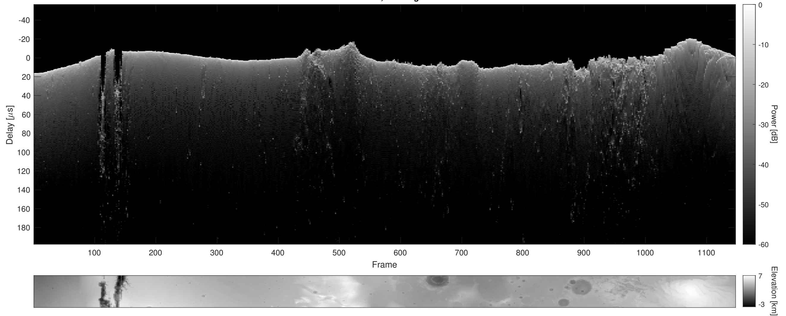
Orbit 13190, Cluttergram
