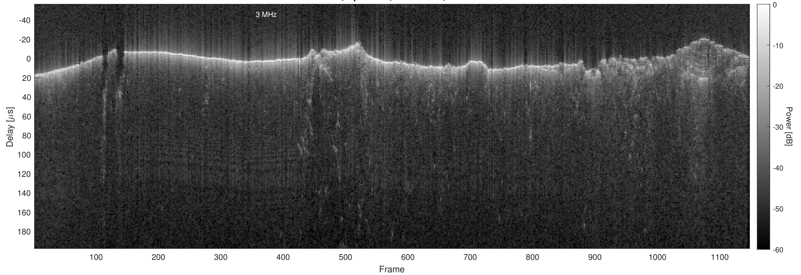
Orbit 13190, Optimized, No Window, Channel 2
