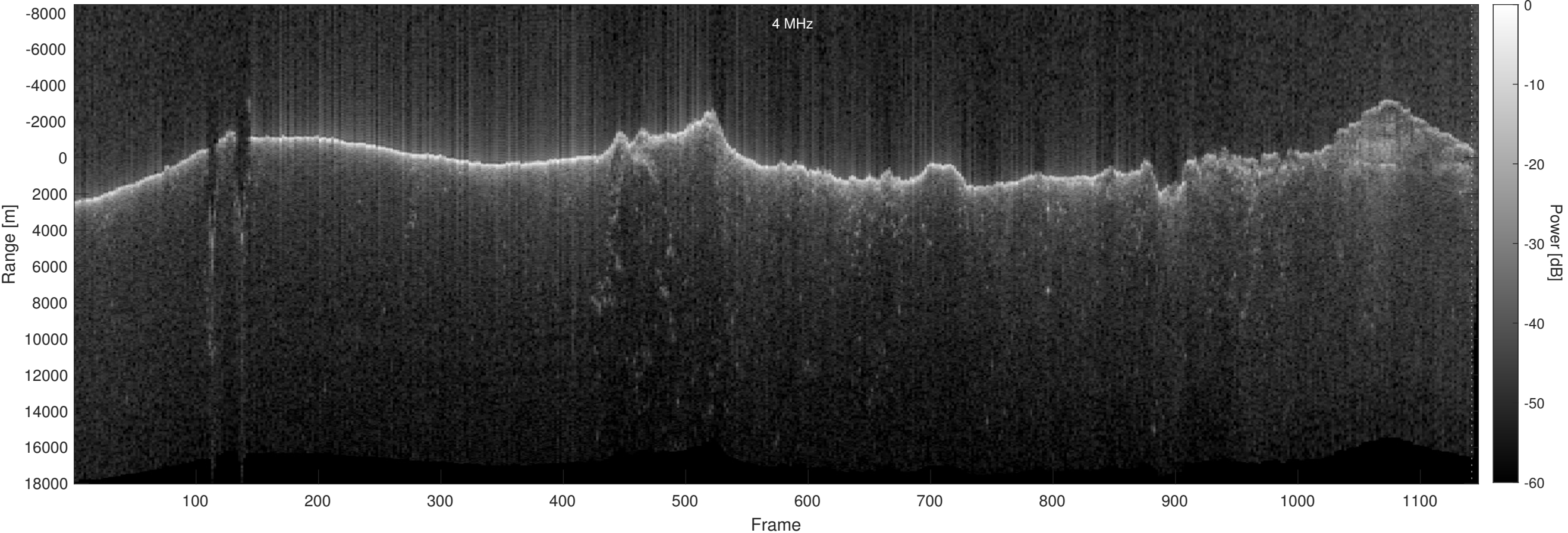
Orbit 13190, Optimized, No Window, Depth-Corrected, Channel 2
