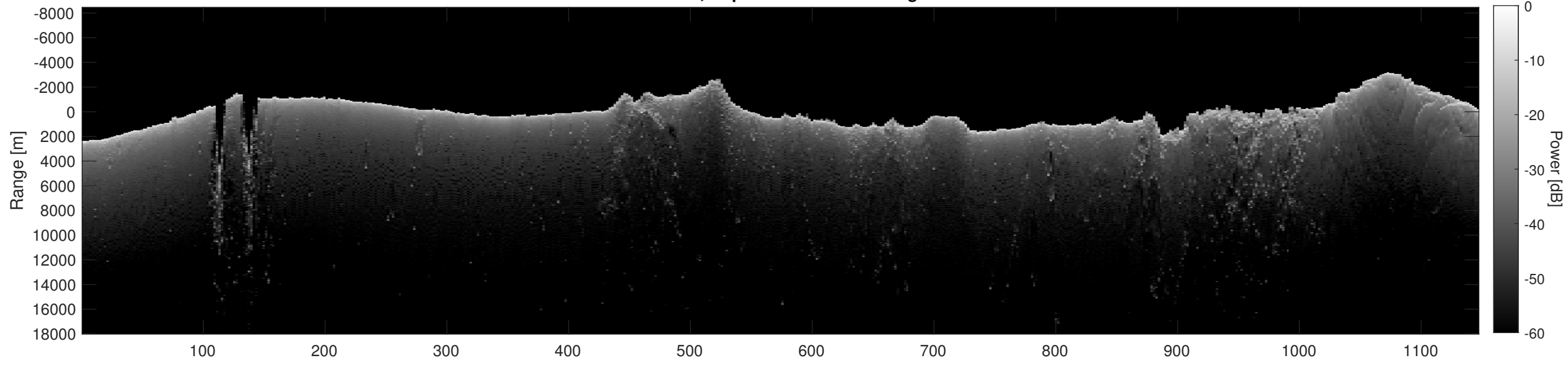
Orbit 13190, Depth-Corrected Cluttergram
