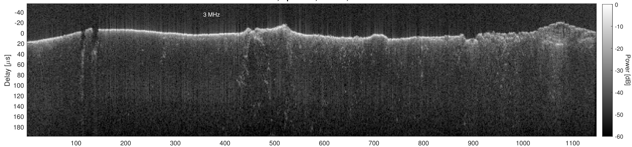
Orbit 13190, Cluttergram
