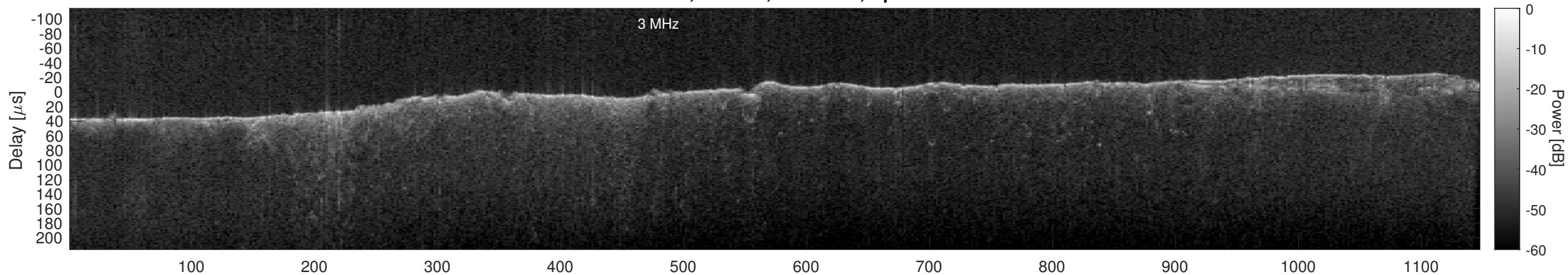
Orbit 13191, Cluttergram
