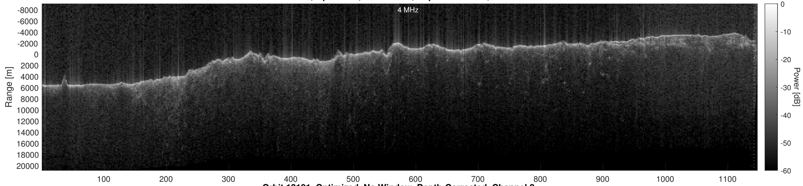
Orbit 13191, Optimized, No Window, Depth-Corrected, Channel 2
