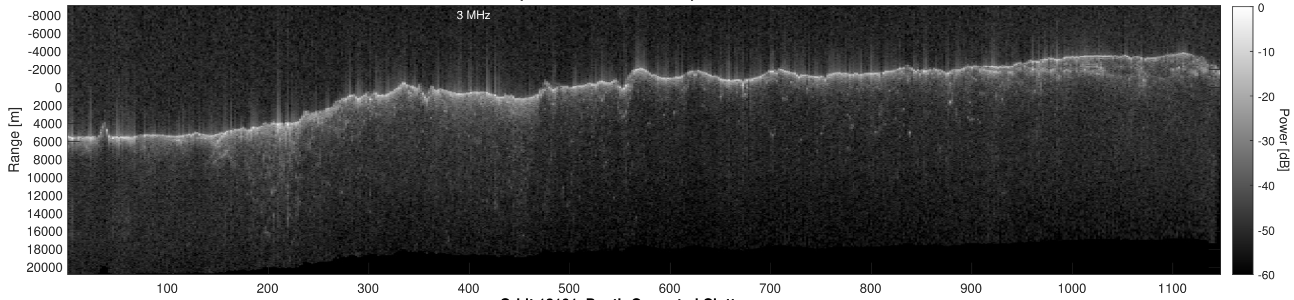
Orbit 13191, Depth-Corrected Cluttergram
