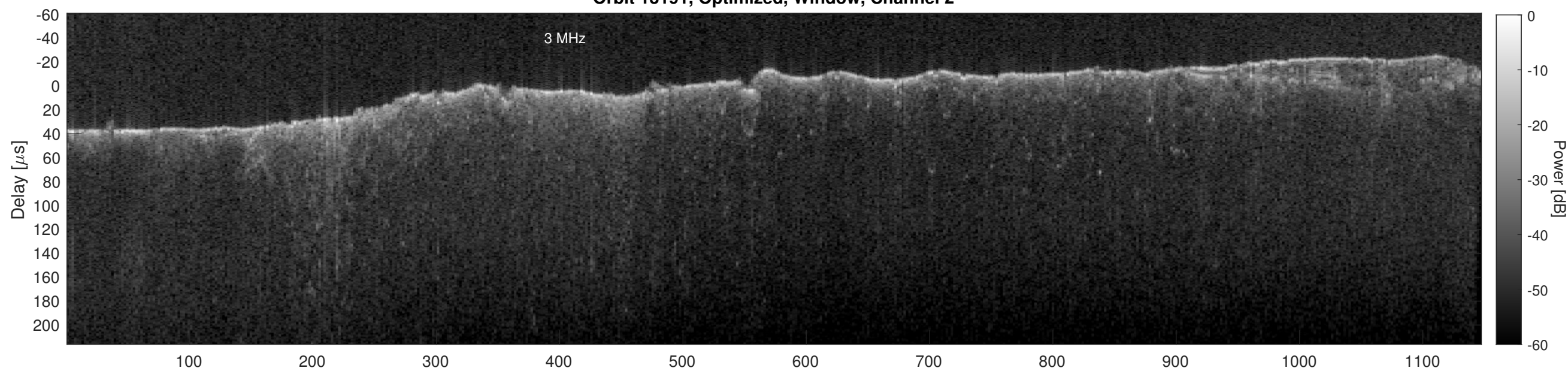
Orbit 13191, Cluttergram
