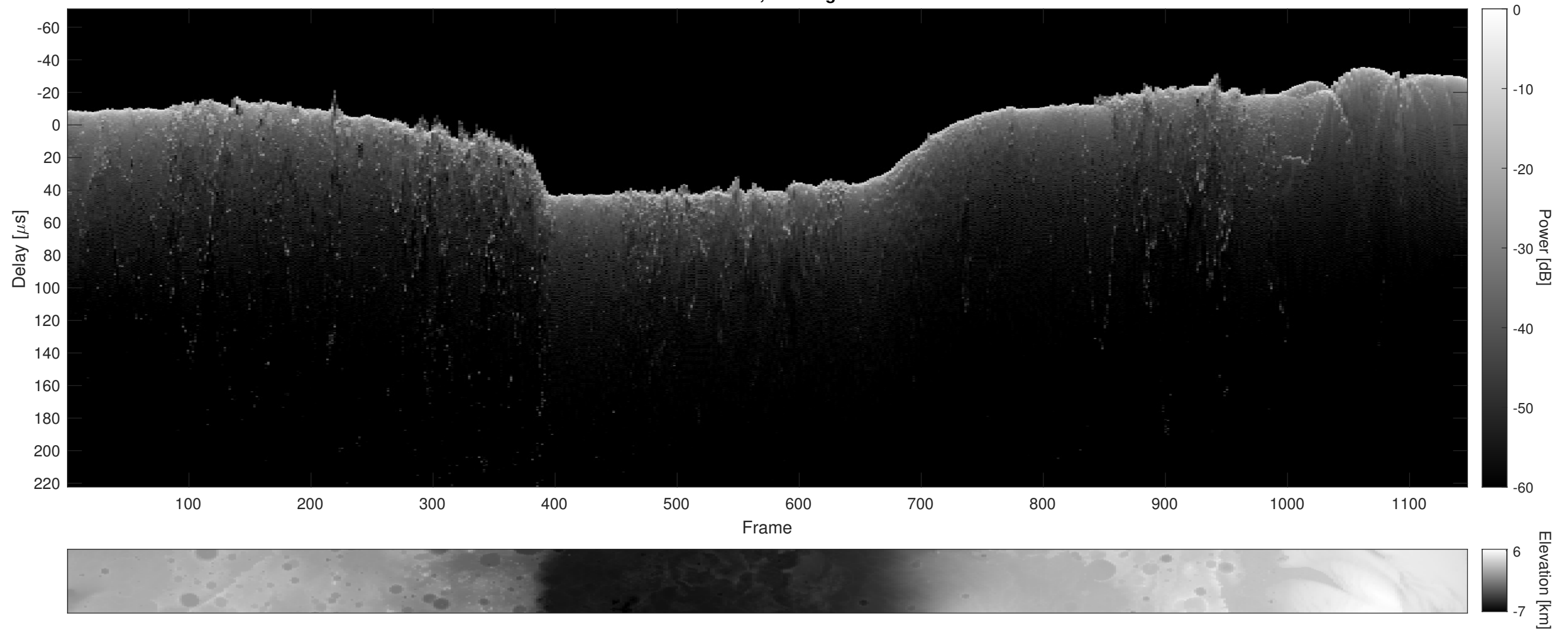
Orbit 13192, Cluttergram
