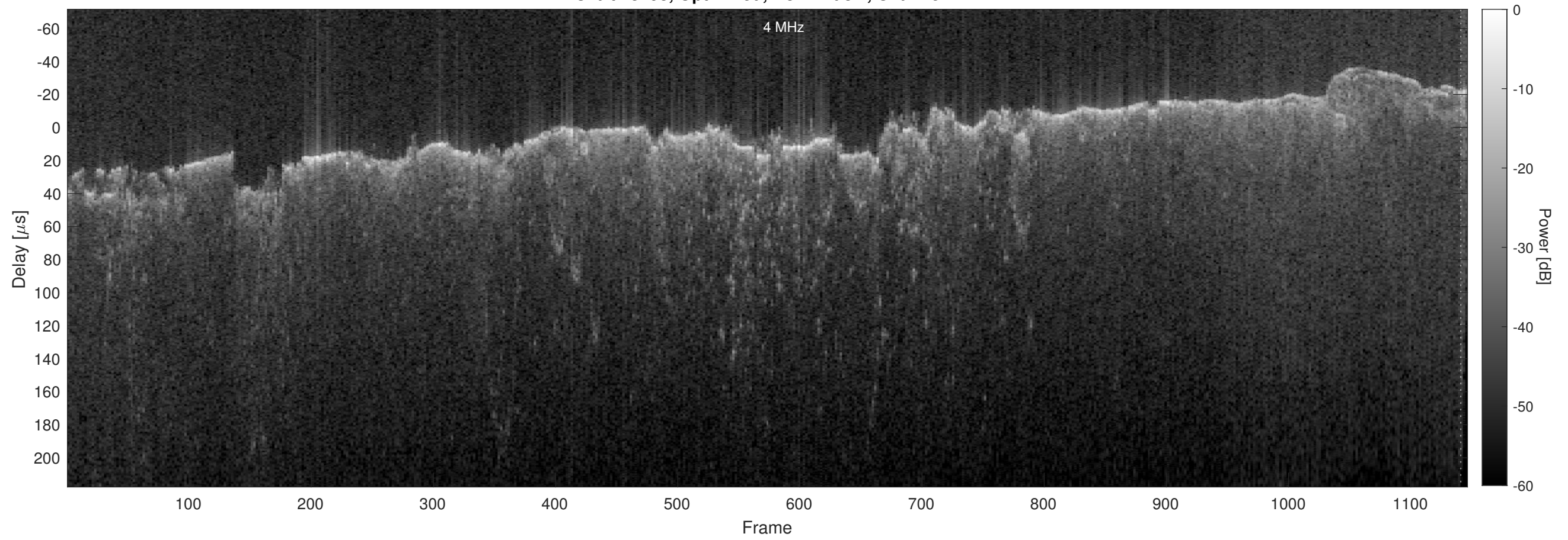
Orbit 13193, Optimized, No Window, Channel 2
