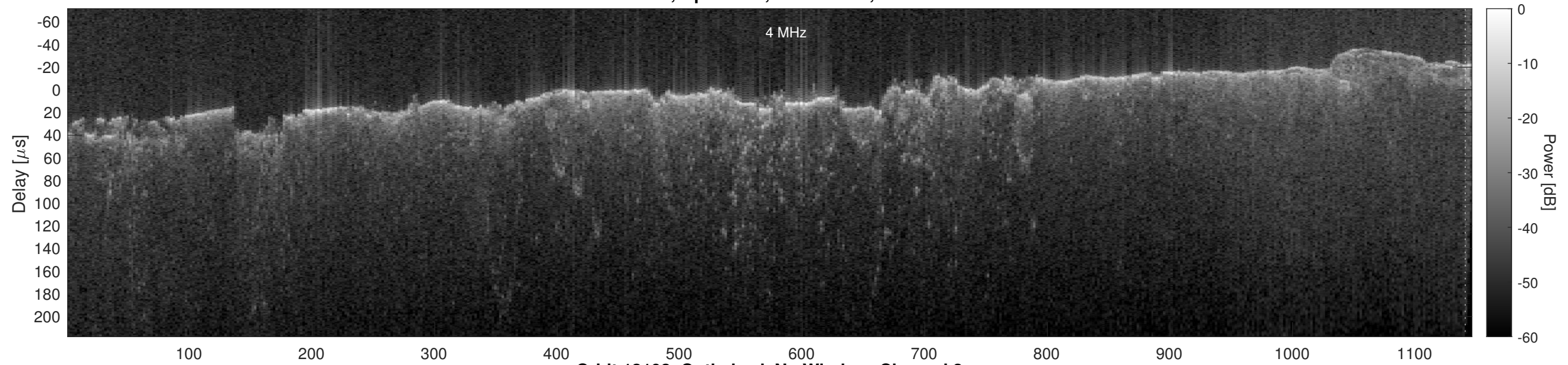
Orbit 13193, Optimized, No Window, Channel 2
