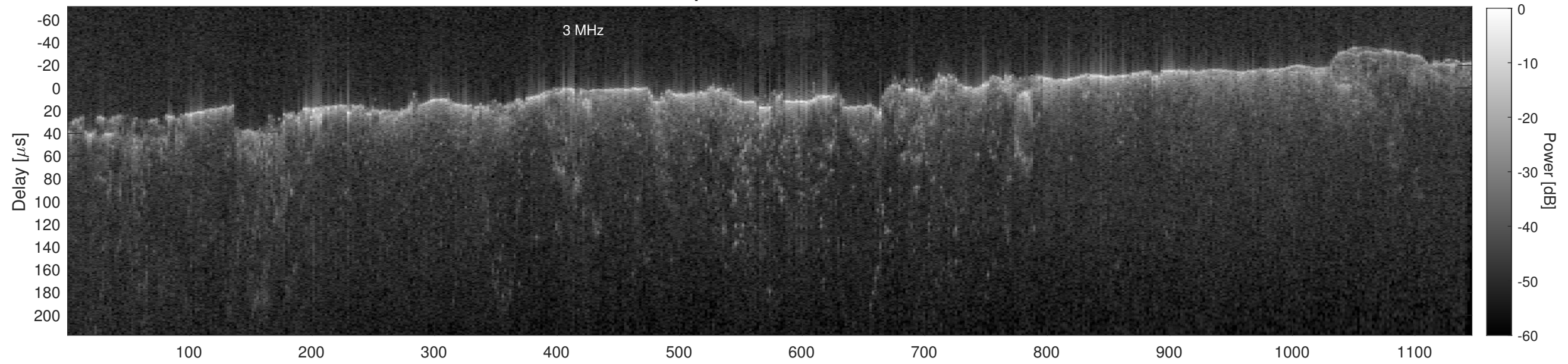
Orbit 13193, Cluttergram
