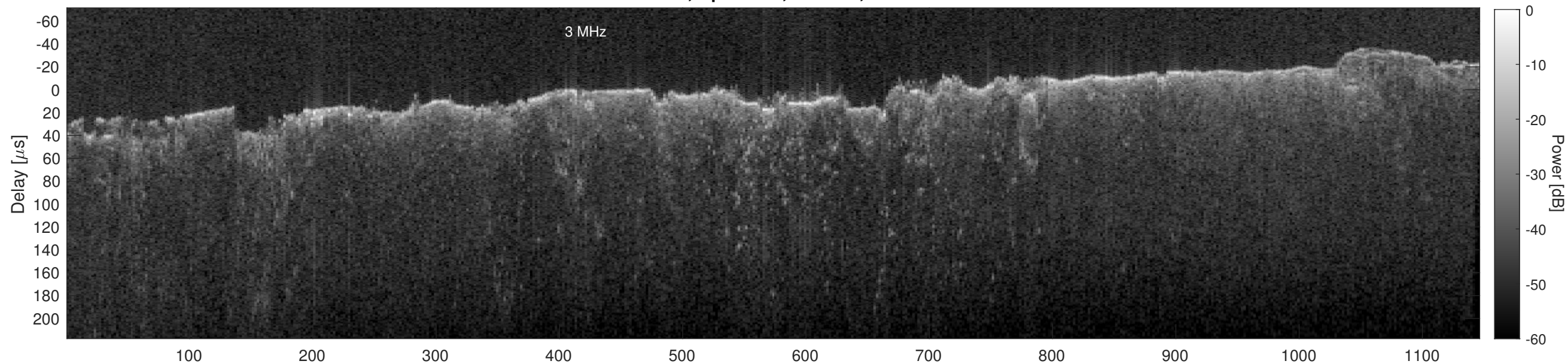
Orbit 13193, Cluttergram
