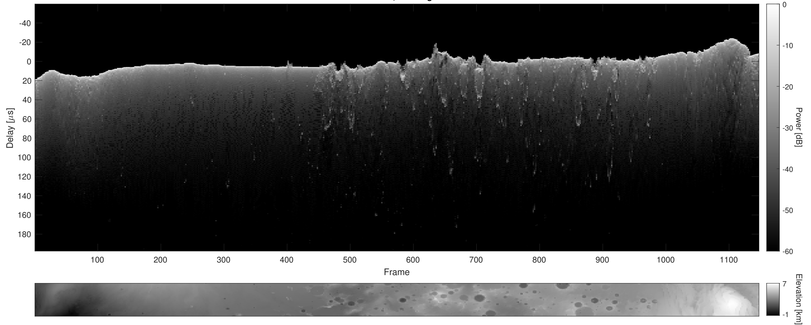
Orbit 13194, Cluttergram
