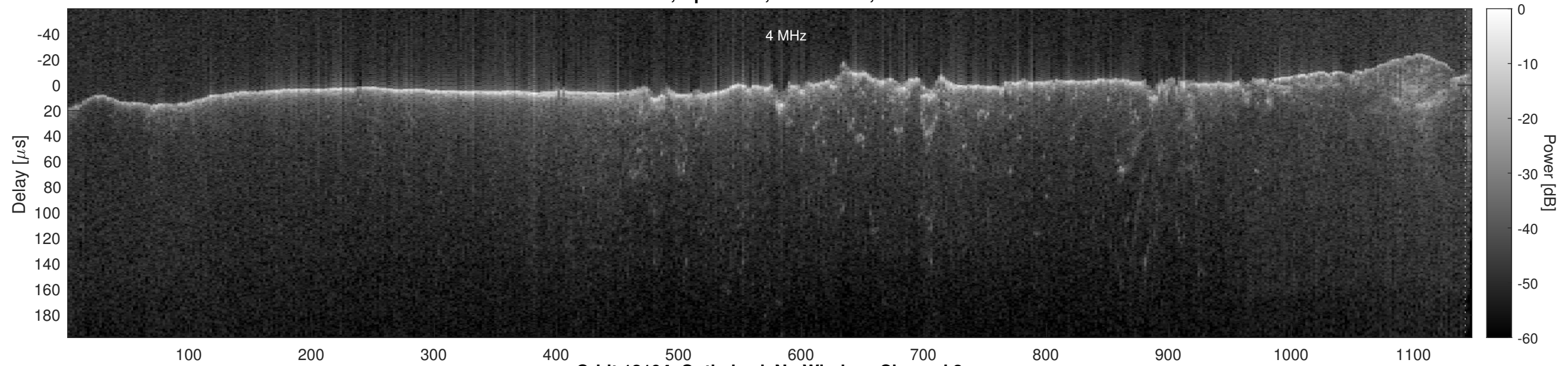
Orbit 13194, Optimized, No Window, Channel 2
