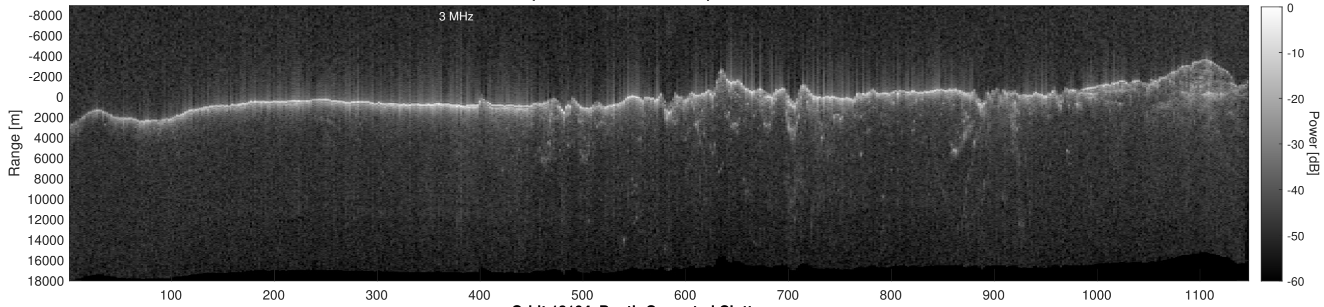
Orbit 13194, Depth-Corrected Cluttergram
