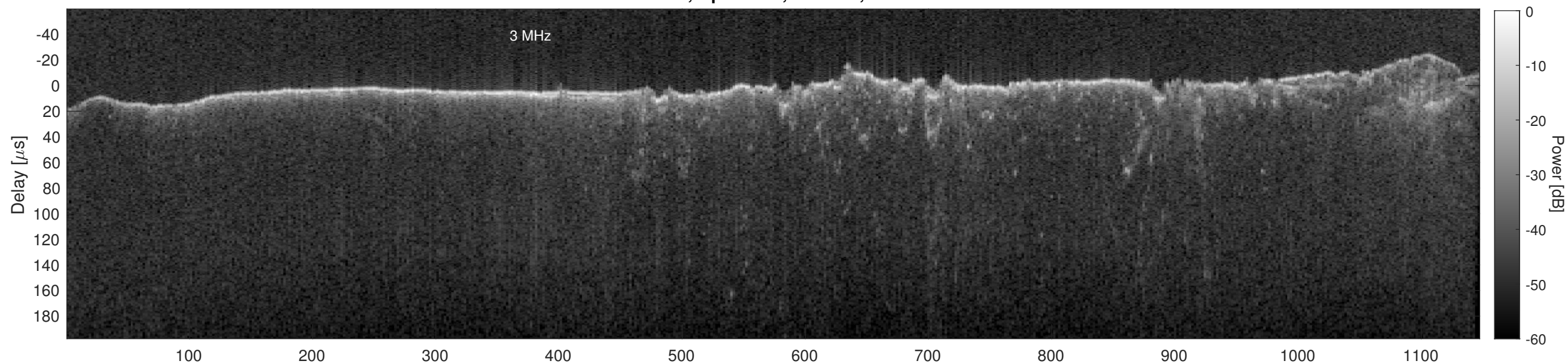
Orbit 13194, Cluttergram
