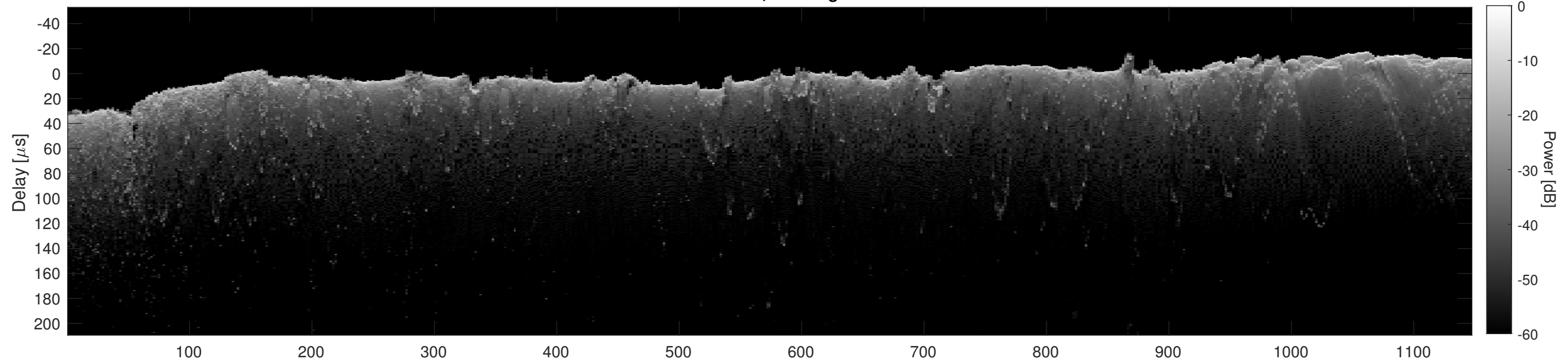
Orbit 13195, Cluttergram
