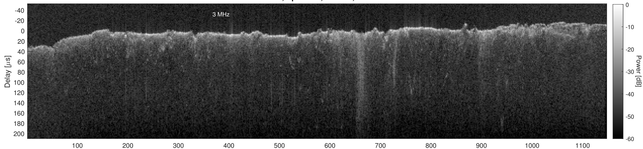
Orbit 13195, Cluttergram
