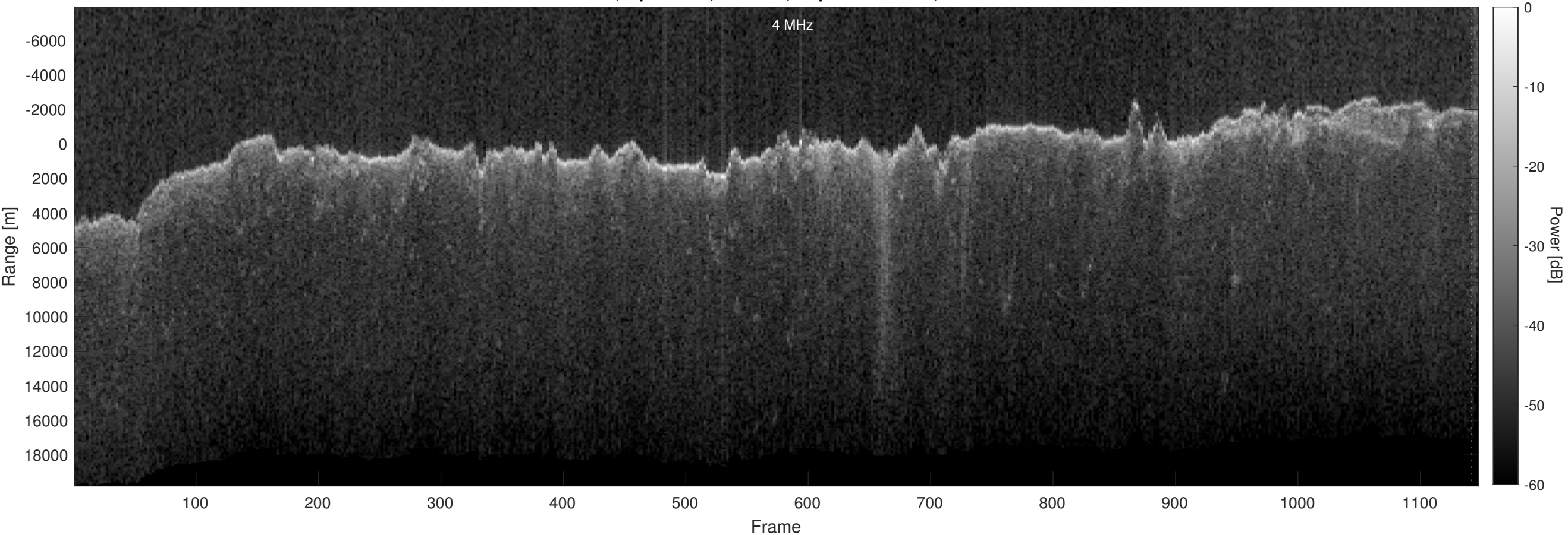
Orbit 13195, Optimized, Window, Depth-Corrected, Channel 2
