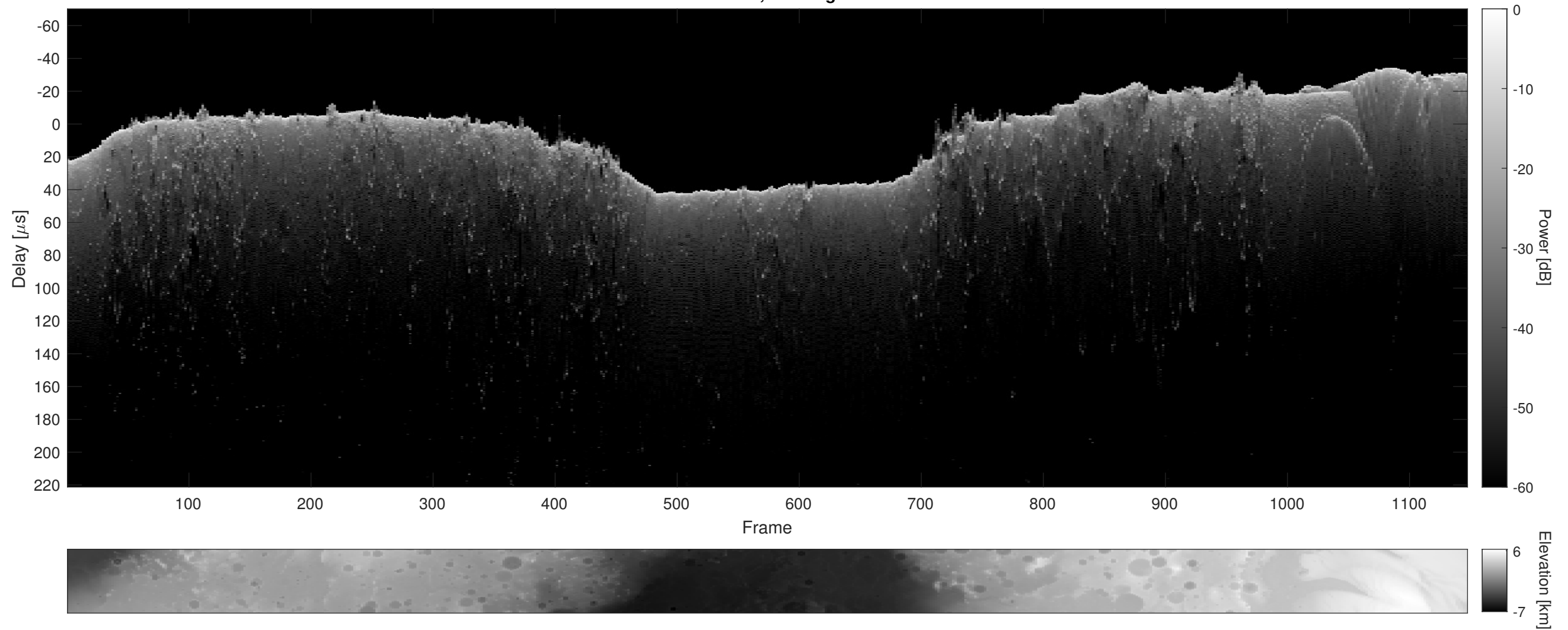
Orbit 13206, Cluttergram
