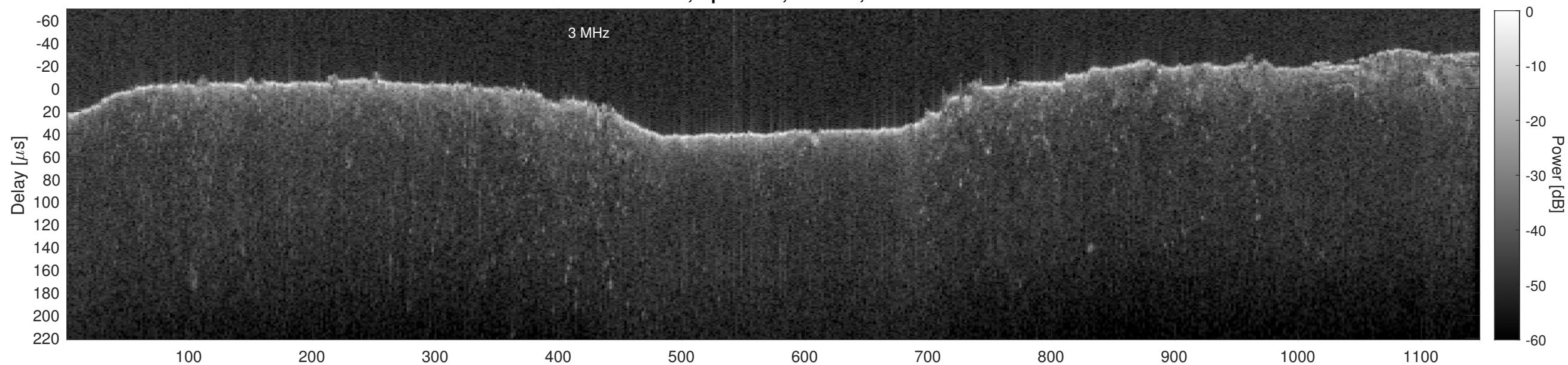
Orbit 13206, Cluttergram
