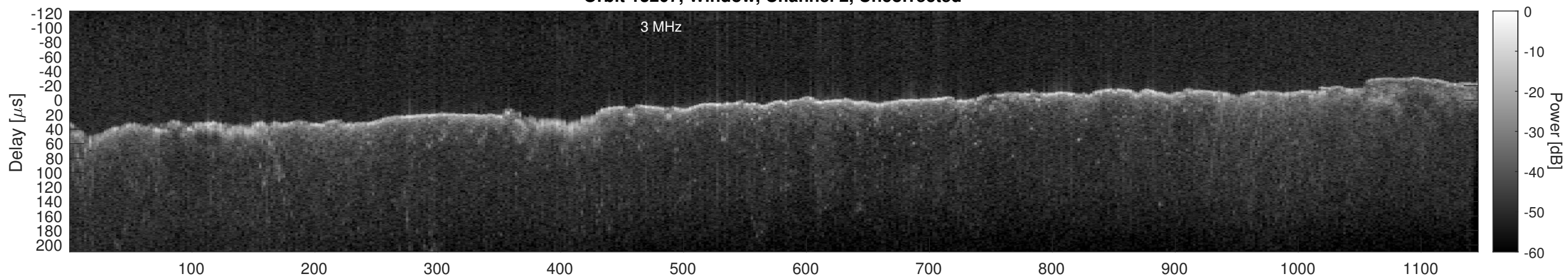
Orbit 13207, Window, Channel 2, Chapman
