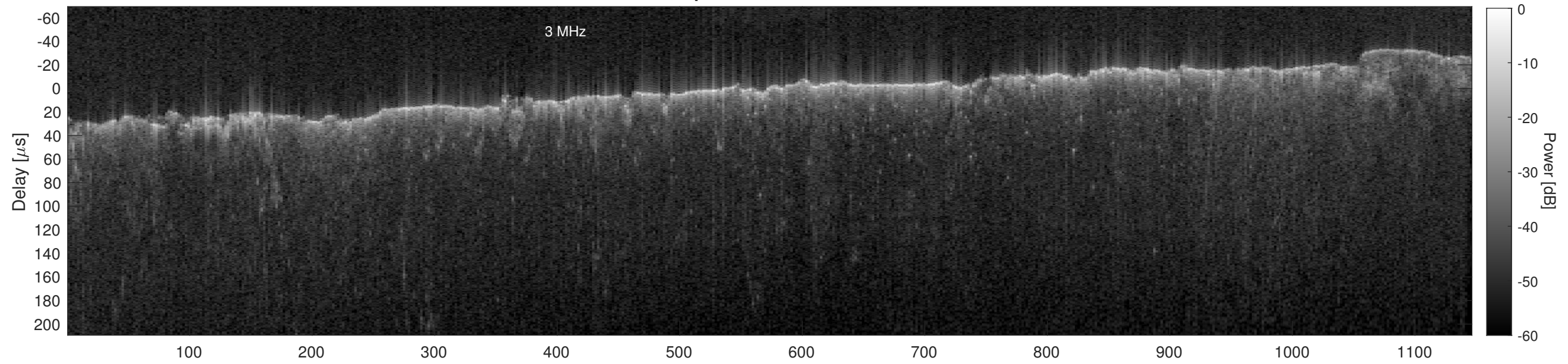
Orbit 13207, Cluttergram
