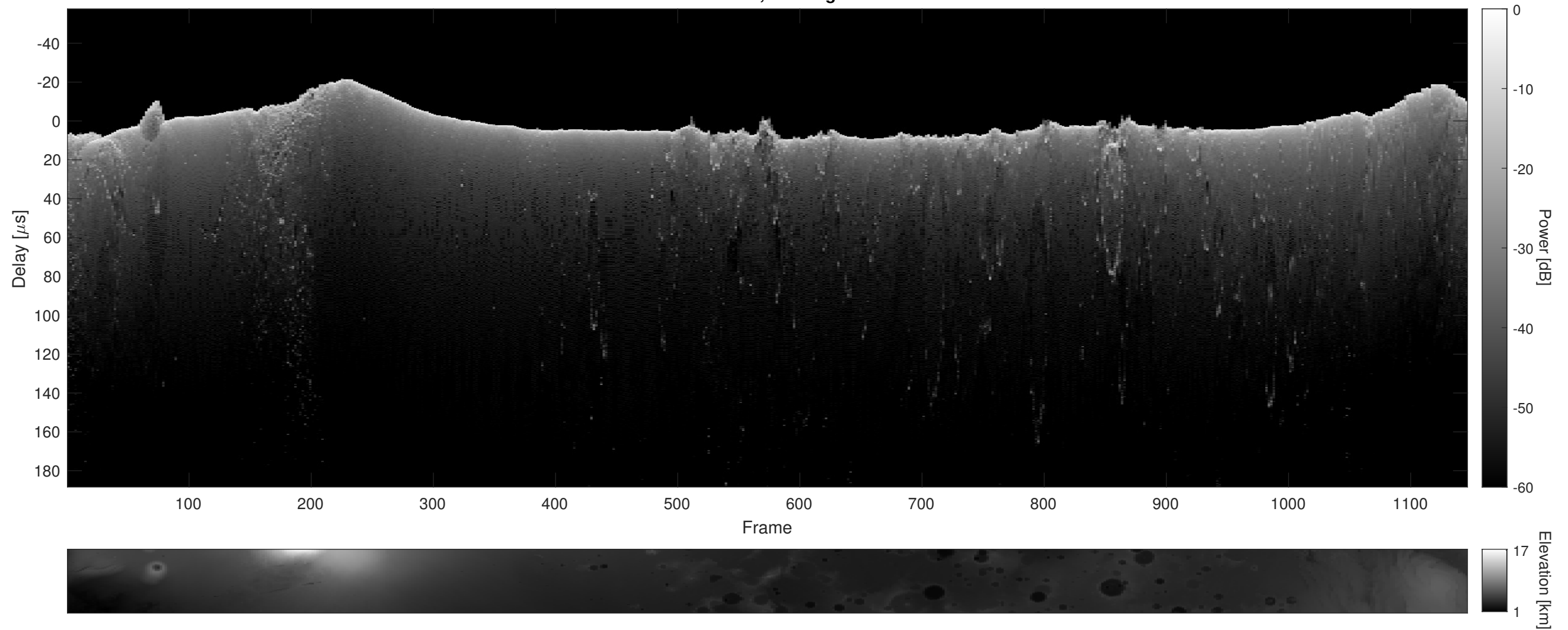
Orbit 13208, Cluttergram
