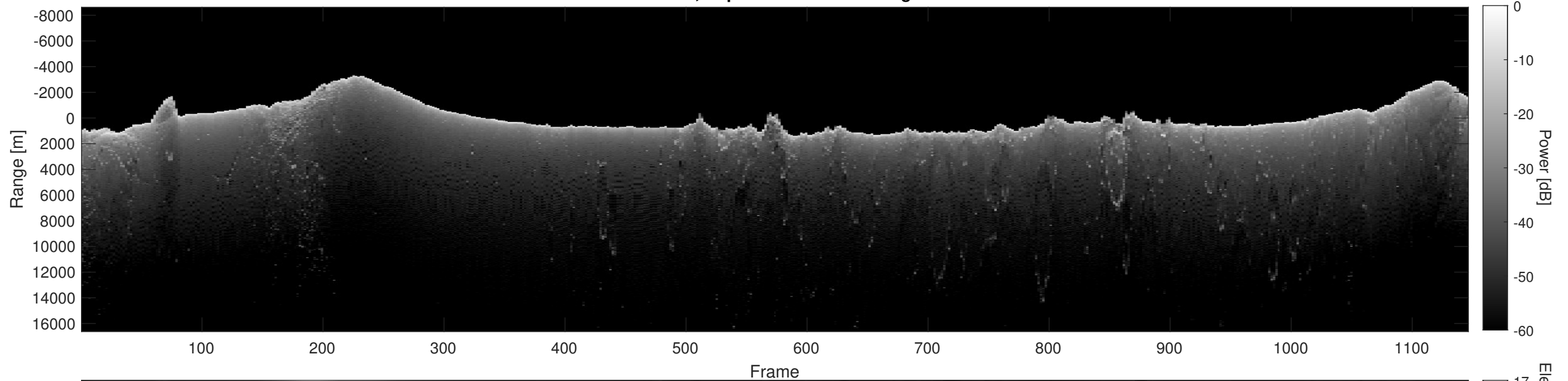
Orbit 13208, Depth-Corrected Cluttergram
