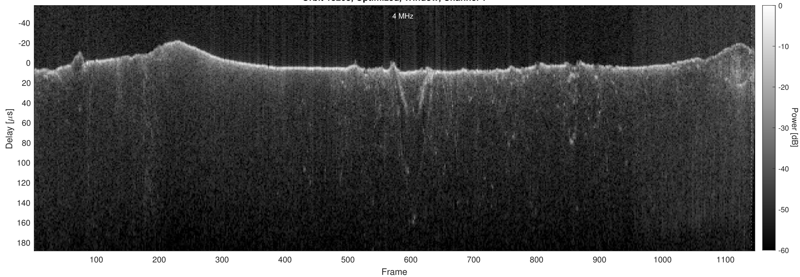
Orbit 13208, Optimized, Window, Channel 2
