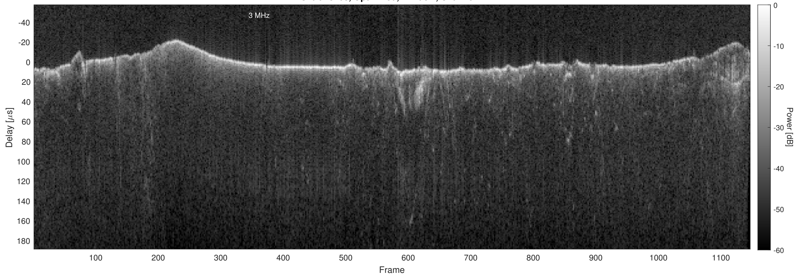
Orbit 13208, Optimized, Window, Channel 2
