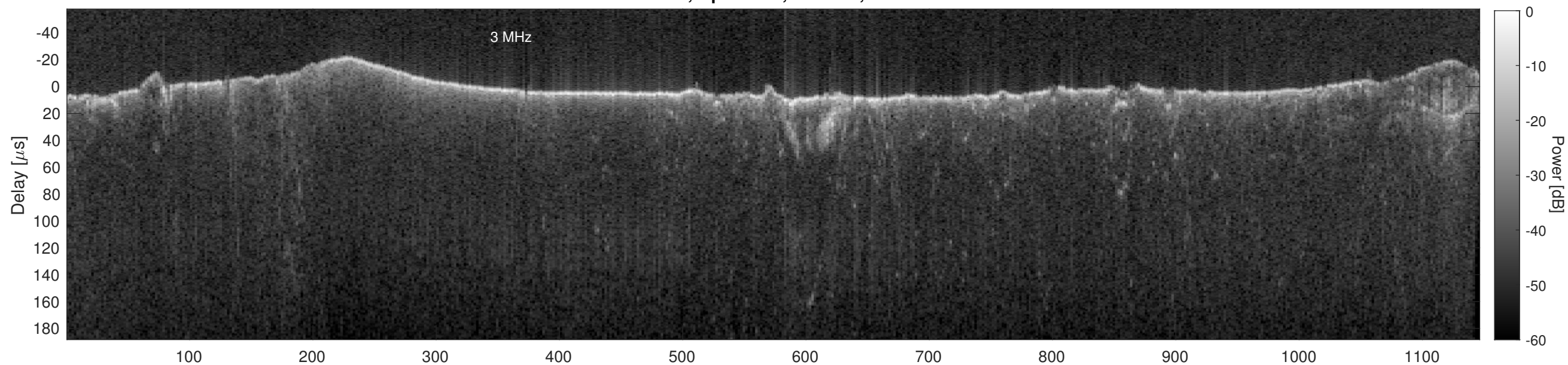
Orbit 13208, Cluttergram
