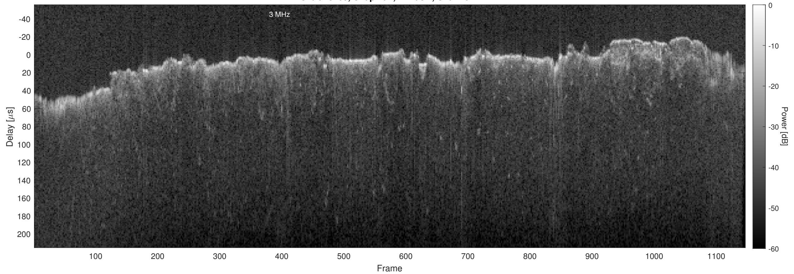
Orbit 13209, Chapman, Window, Channel 2
