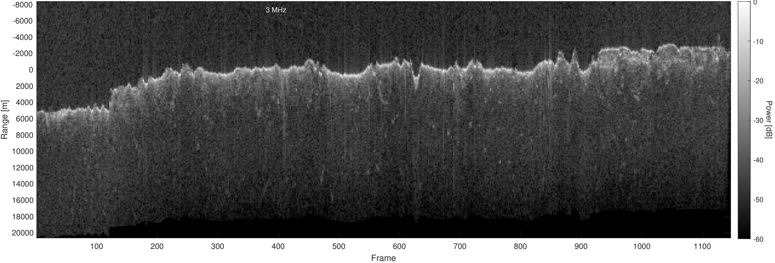
Orbit 13209, Optimized, Window, Depth-Corrected, Channel 2
