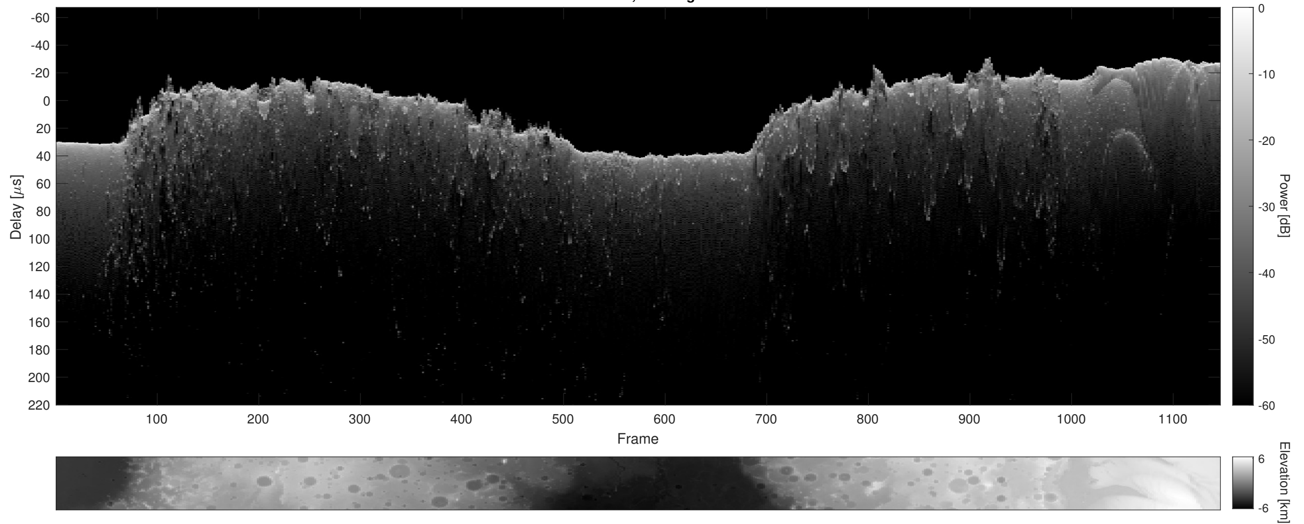
Orbit 13213, Cluttergram
