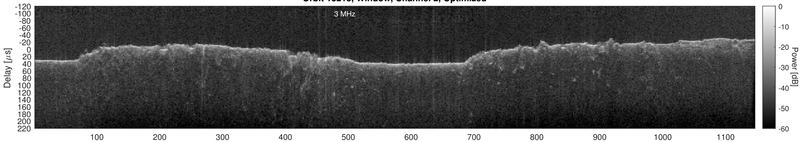
Orbit 13213, Cluttergram
