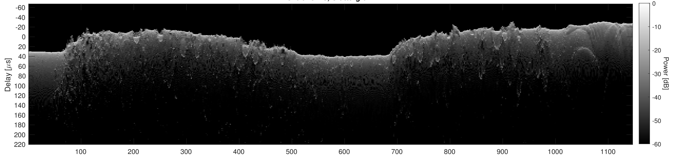
Orbit 13213, Cluttergram
