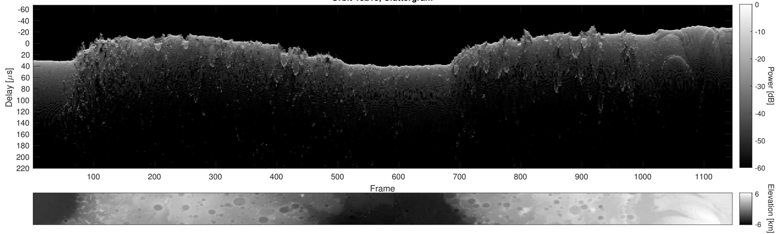
Orbit 13213, Cluttergram
