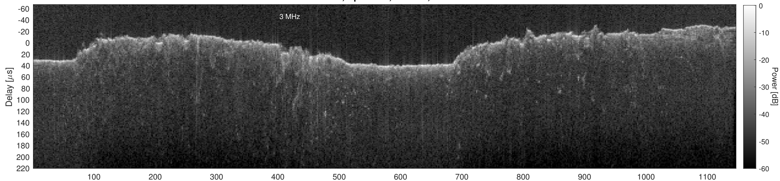
Orbit 13213, Cluttergram
