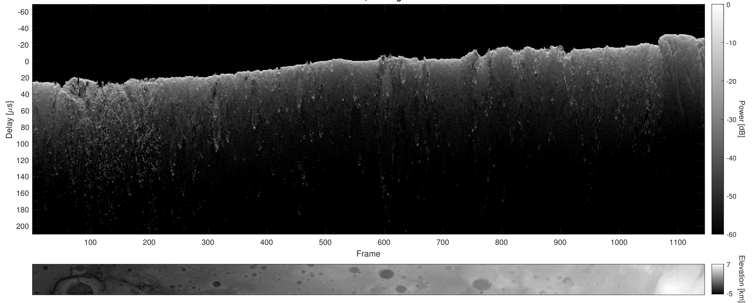
Orbit 13214, Cluttergram
