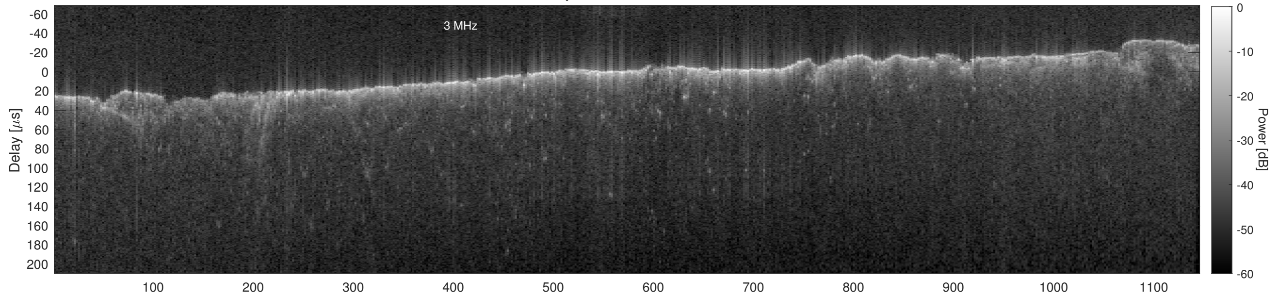
Orbit 13214, Cluttergram
