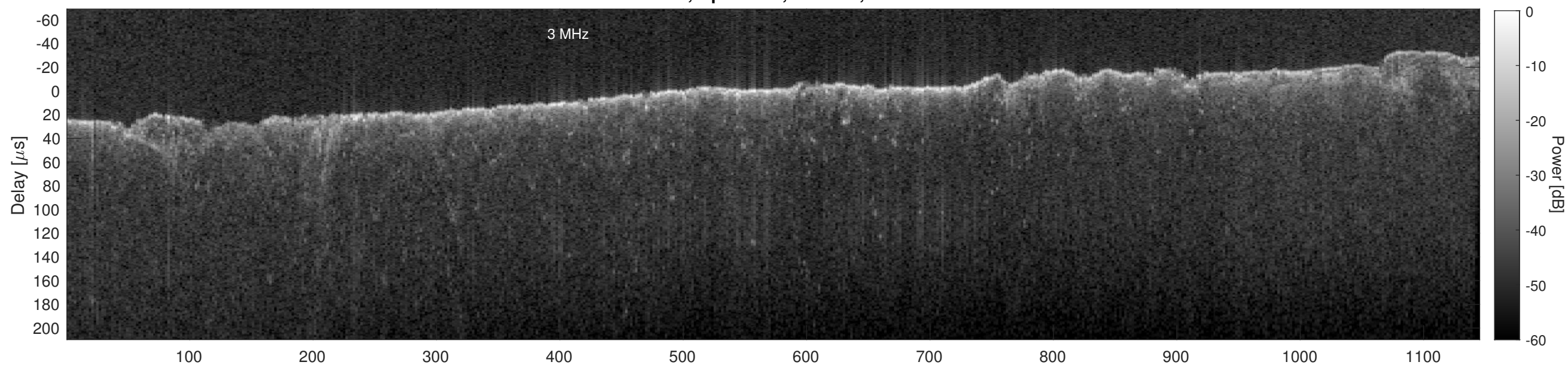
Orbit 13214, Cluttergram
